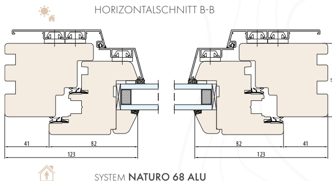
SYSTEM NATURO 68 ALU RENO LINE
